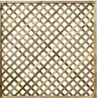
Heavy Diamond Lattice (HDL)
